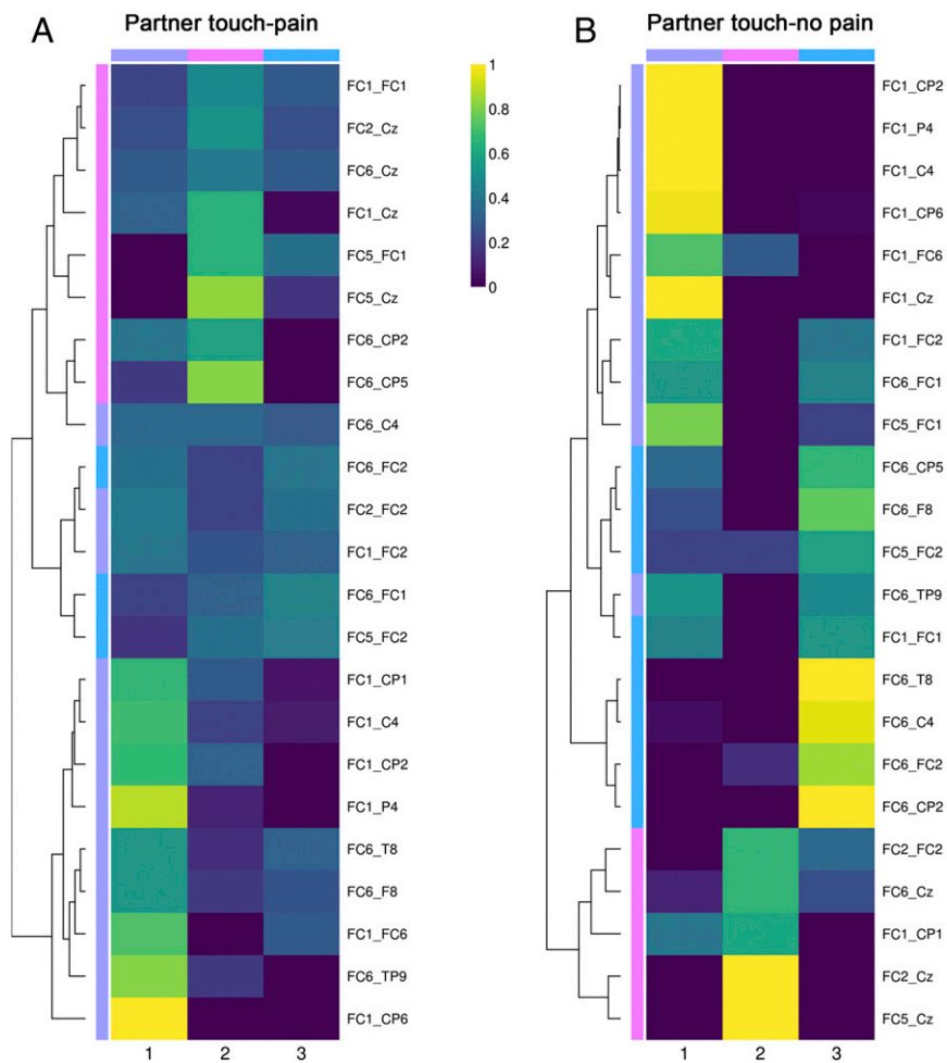
Fig. 3. Heatmaps of the three-cluster solution for significant interbrain coupling links during pain: (A) partner touch–pain condition; (B) partner touch–no-pain condition. The colors reflect coupling link loadings for each cluster. The tree diagram (dendograms in the left part of the plots) illustrates the arrangement of the clusters produced by hierarchical clustering. The first and second electrode names separated by an underscore (right side of each heatmap) represent the target and observer EEG channels that take part in the brain-to-brain coupling.
